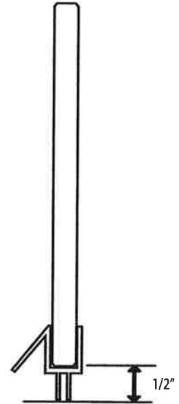
Vertical Detail Through DOOR
