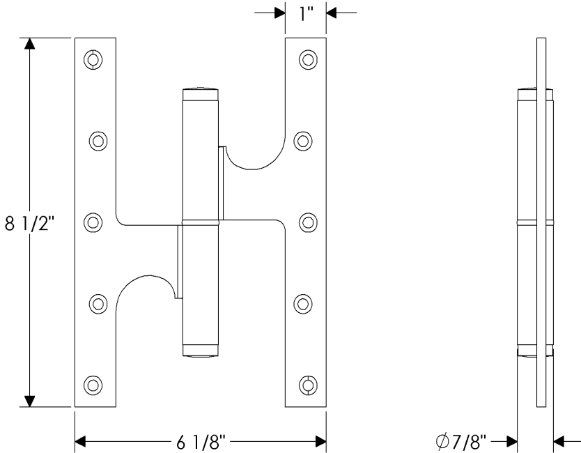
PHNG8.5x6.125 Paumelle Hinge 8 1/2" x 6 1/8"
