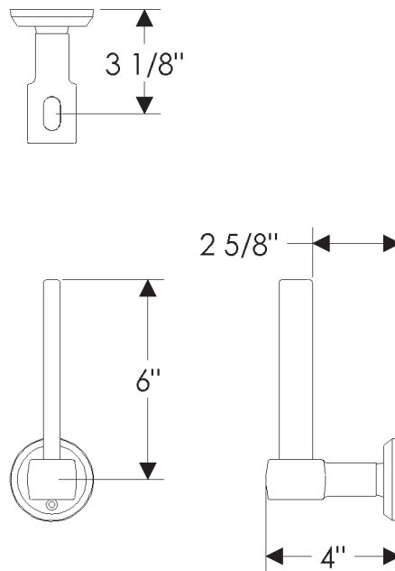
TP4 Tempo Vertical Toilet Paper Holder
